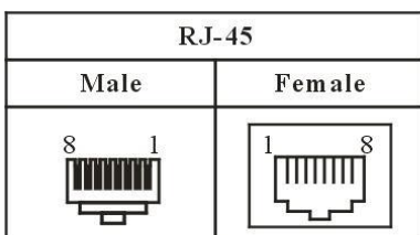
Figure1: RJ-45 pin-out
