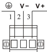
Figure 1 Power input terminal
